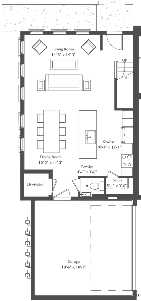
FIRST FLOOR
